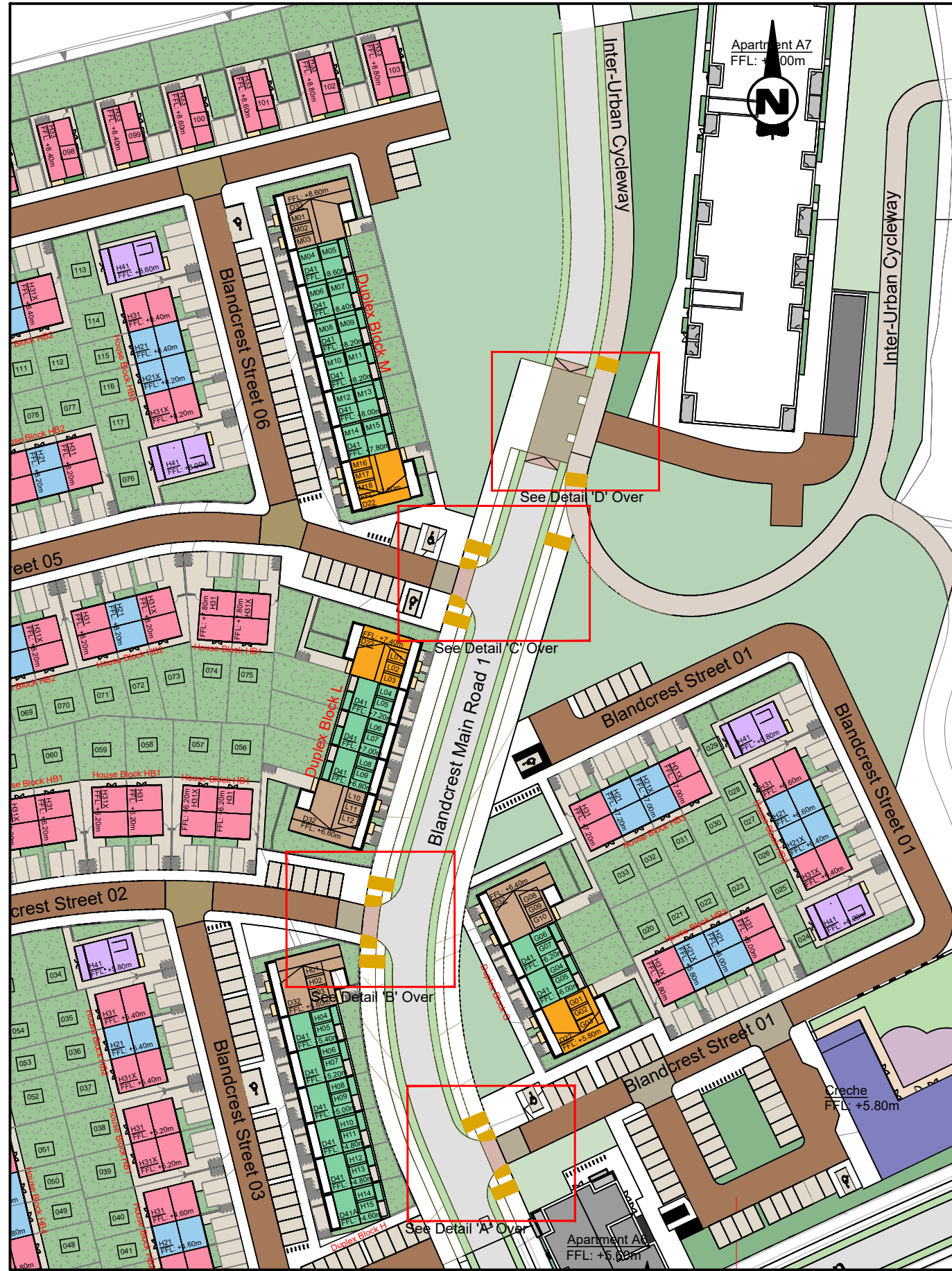
1:500 Layout Plan
